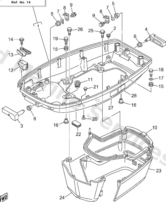
Fig. 14, BOTTOM COWLING Ref. No. 14
