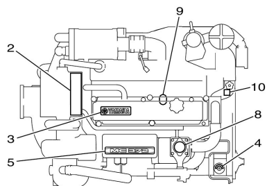
ENGINE UPPER SIDE
