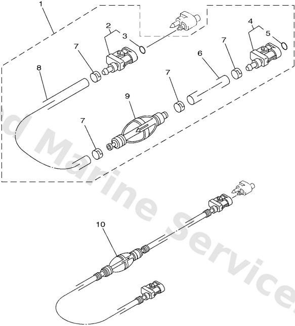
FUEL PIPE
