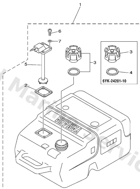
FUEL TANK (25L)
