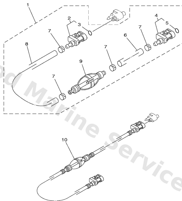
FUEL PIPE
