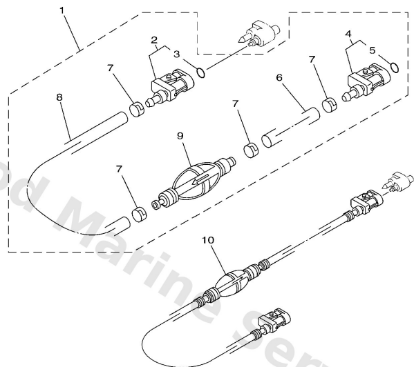
PRIMARY PUMP
