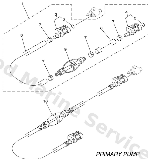
FUEL PIPE
