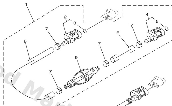
FUEL PIPE
