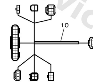
2ND STATION HELM HARNESS FOR TWIN/TRIPLE/QUAD
