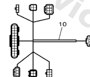
2ND STATION HELM HARNESS FOR TWIN/TRIPLE/QUAD
