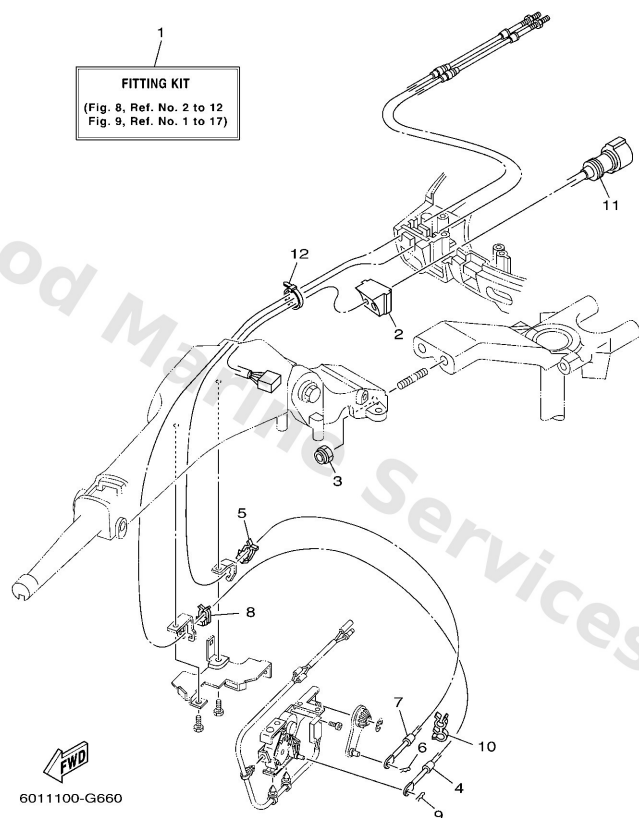
6X4 TILLER HANDLE FITTING KIT (F40)
