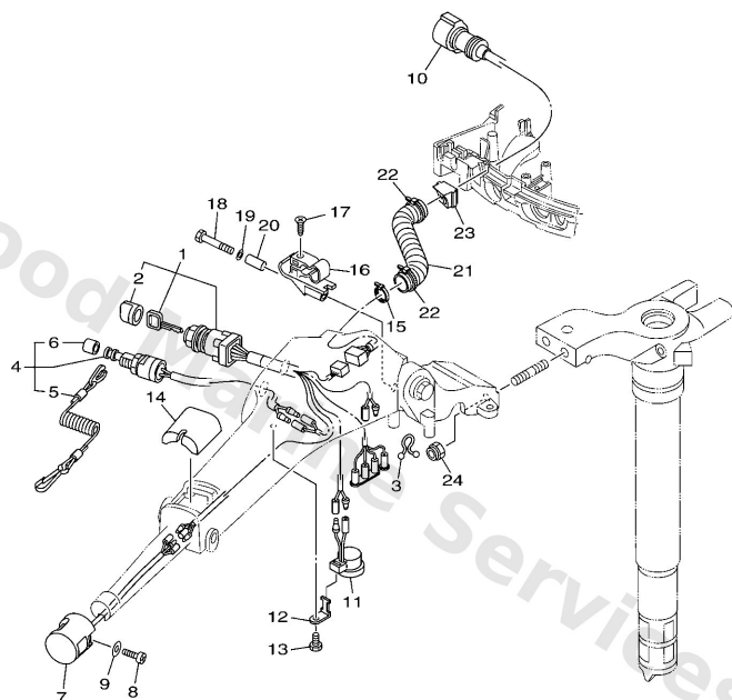
6X4 TILLER HANDLE COMPLETE (F25)
