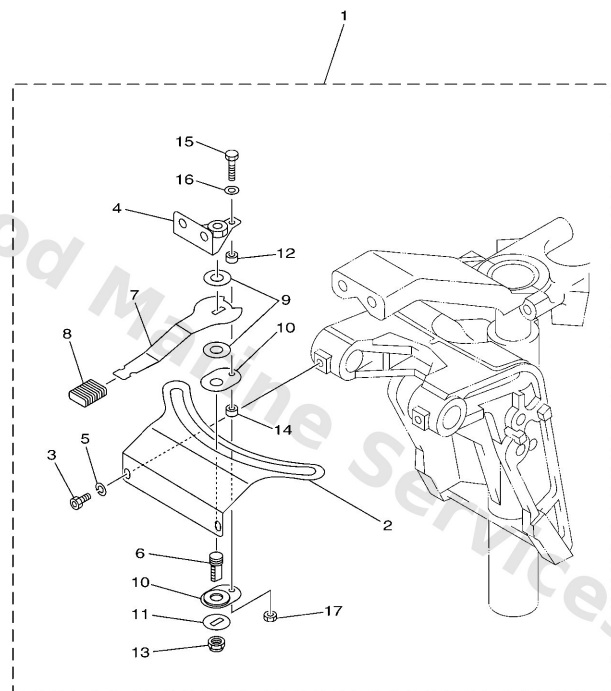
6X4 TILLER HANDLE FITTING KIT STEERING FRICTION (F50,T50,F60,T60)
