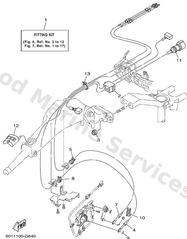
6X4 TILLER HANDLE FITTING KIT (F50,T50,F60,T60)
