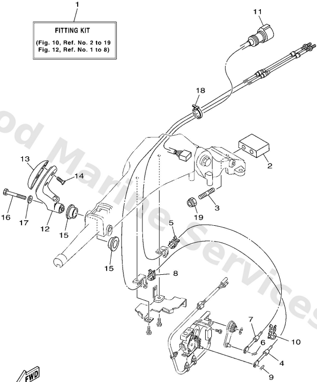
6X4 TILLER HANDLE FITTING KIT (90)
