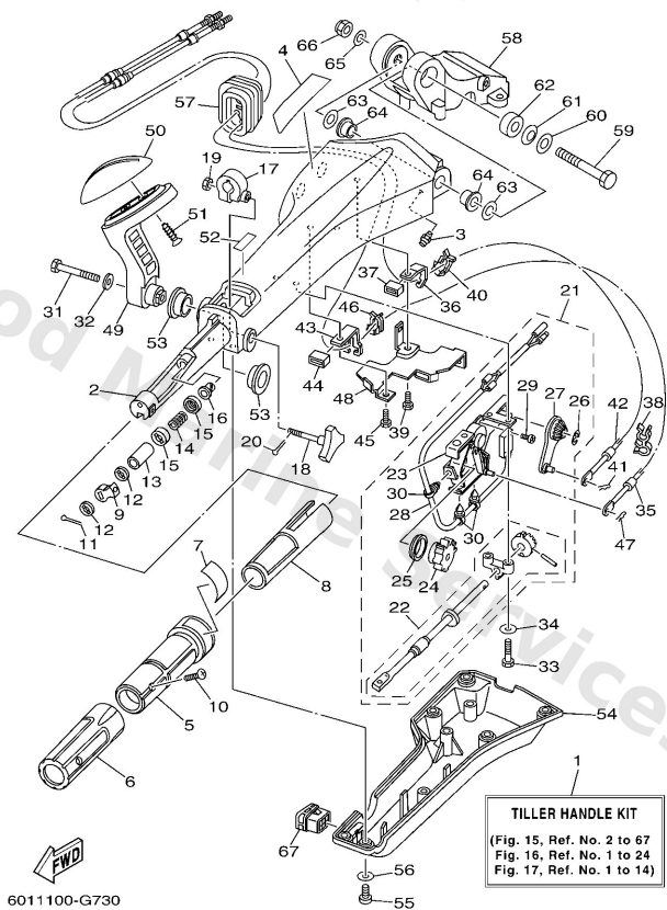
6X4 TILLER HANDLE COMPLETE (F25)
