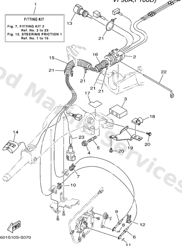
6X4 TILLER HANDLE FITTING KIT (F75B,F80B, VF90A,F100D)
