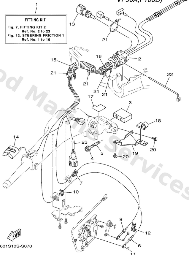
6X4 TILLER HANDLE FITTING KIT (F75B,F80B, VF90A,F100D)
