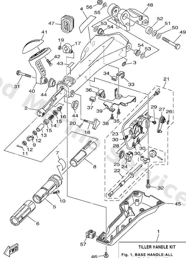
6X4 TILLER HANDLE KIT (F20F-F130A)
