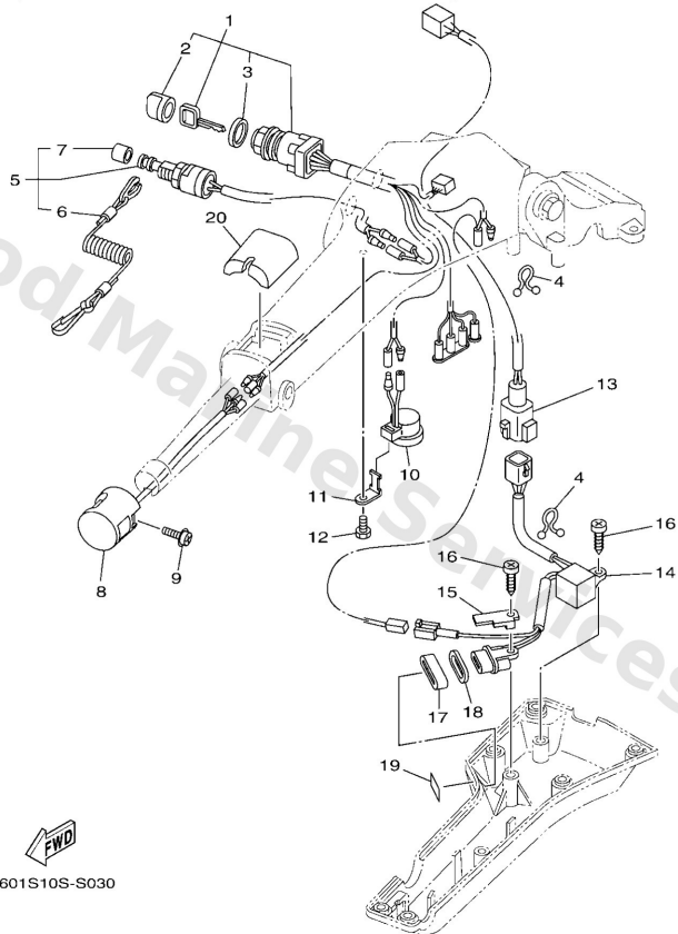
6X4 TILLER HANDLE KIT (F20F-F130A FOR EUROPE, OCEANIA)
