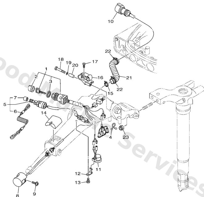
6X4 TILLER HANDLE KIT (F25A,F25B FOR USA,CANADA)
