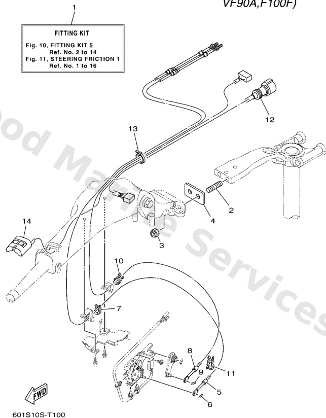
6X4 TILLER HANDLE FITTING KIT (F75B,F80D,F90B, VF90A,F100F)
