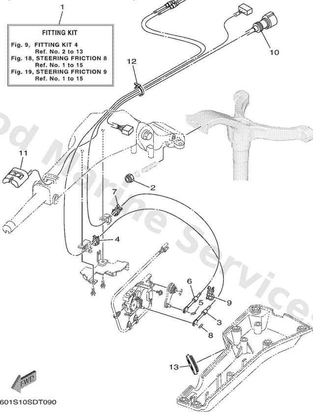
6X4 TILLER HANDLE FITTING KIT (F20B,F20G,F25C,F25G)
