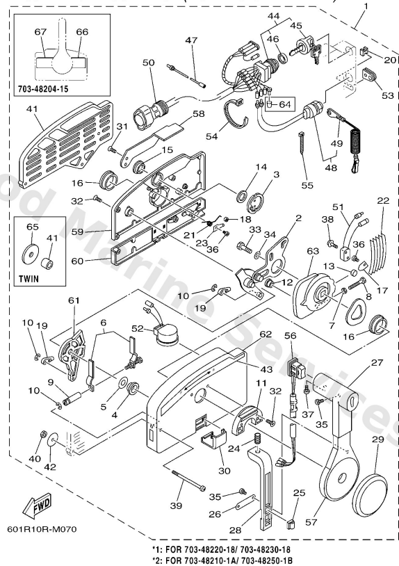
703 REMOTE CONTROL (PULL TO OPEN TYPE)
