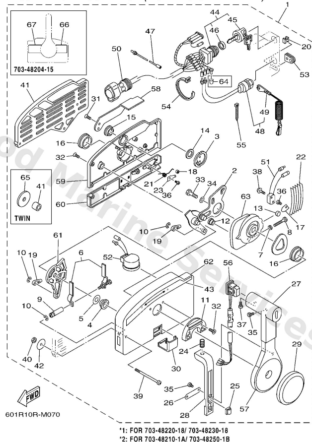
703 REMOTE CONTROL (PULL TO OPEN TYPE)
