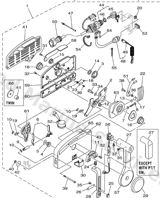
703 REMOTE CONTROL (PUSH TO OPEN TYPE)
