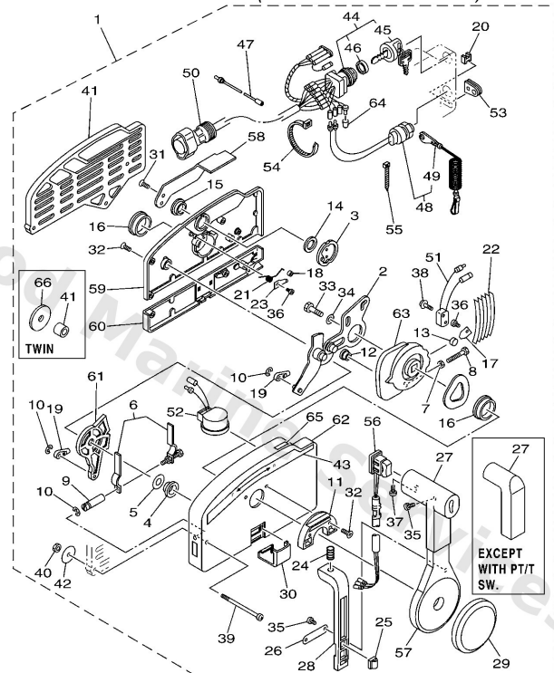
703 REMOTE CONTROL (PUSH TO OPEN TYPE)
