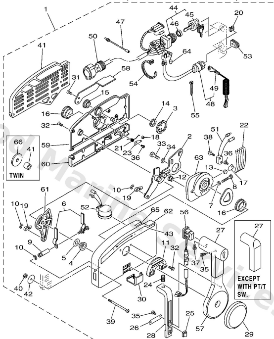
703 REMOTE CONTROL (PUSH TO OPEN TYPE)
