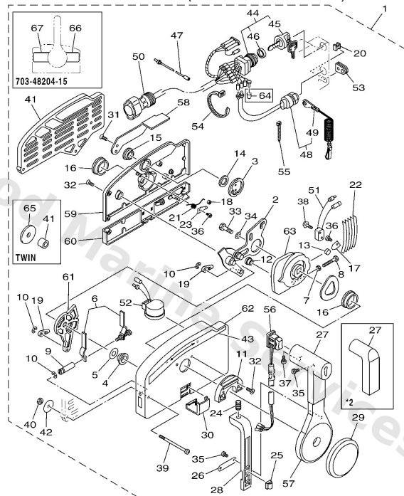
703 REMOTE CONTROL (PULL TO OPEN TYPE)
