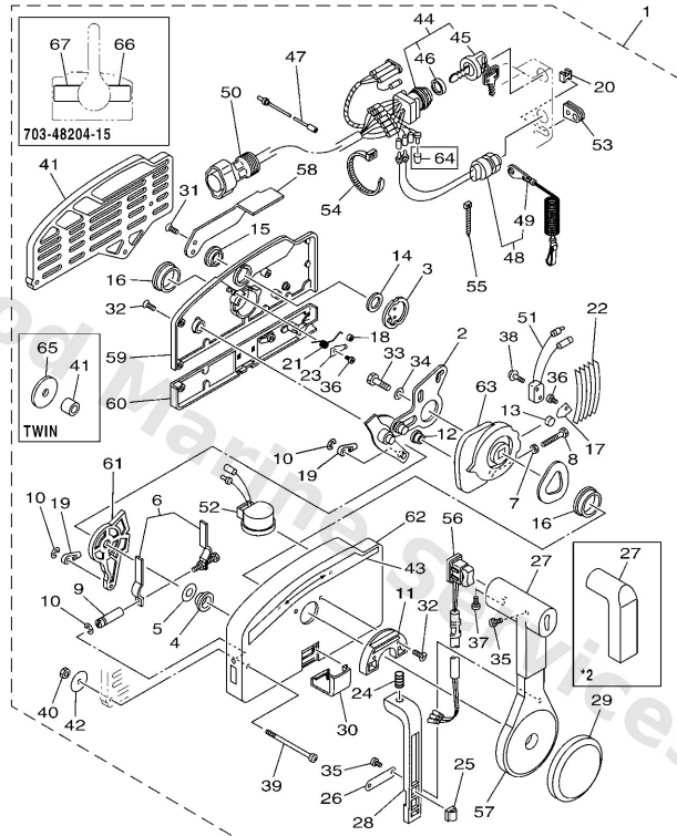
703 REMOTE CONTROL (PULL TO OPEN TYPE)
