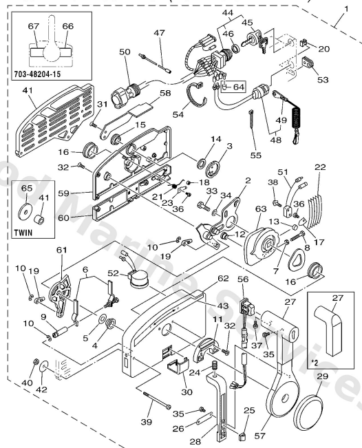
703 REMOTE CONTROL (PULL TO OPEN TYPE)
