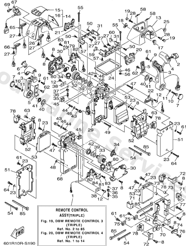
6X6 REMOTE CONTROL (TRIPLE)
