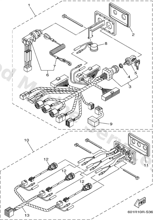
DIGITAL NETWORK SYSTEM-6Y9 (TRIPLE :1 & 2 STATION-MAIN)
