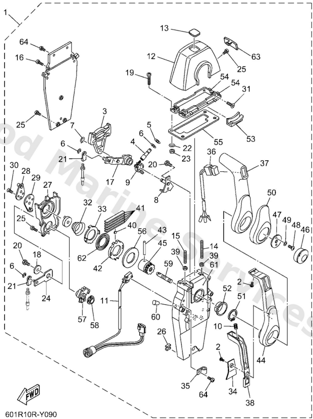
704 REMOTE CONTROL (SINGLE WITH NEUTRAL LOCK)
