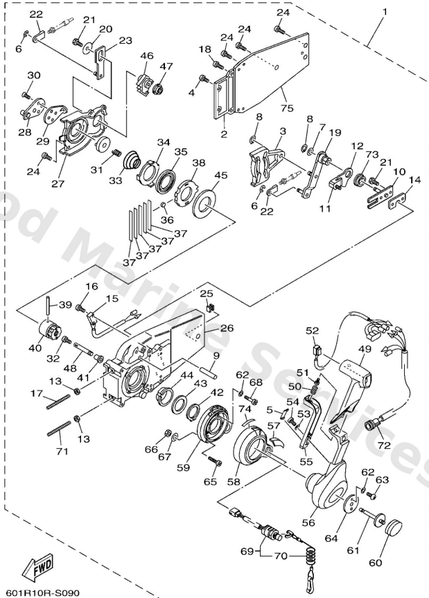
6X3 REMOTE CONTROL (RIGHT MOUNT)
