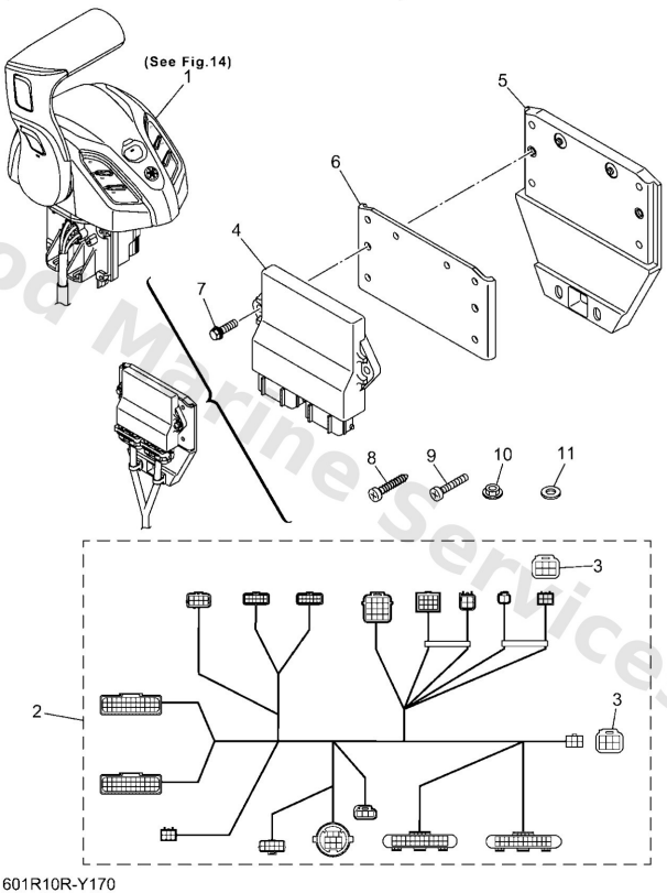
DIGITAL ELECTRONIC CONTROL (SINGLE ENGINE / MAIN STATION)
