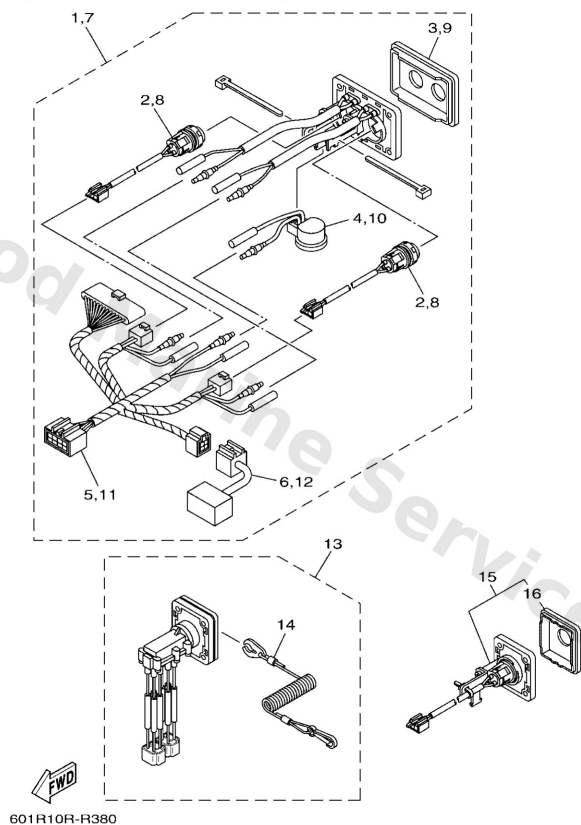
DIGITAL NETWORK SYSTEM-6Y9 (QUAD : 2 STATION-SUB)
