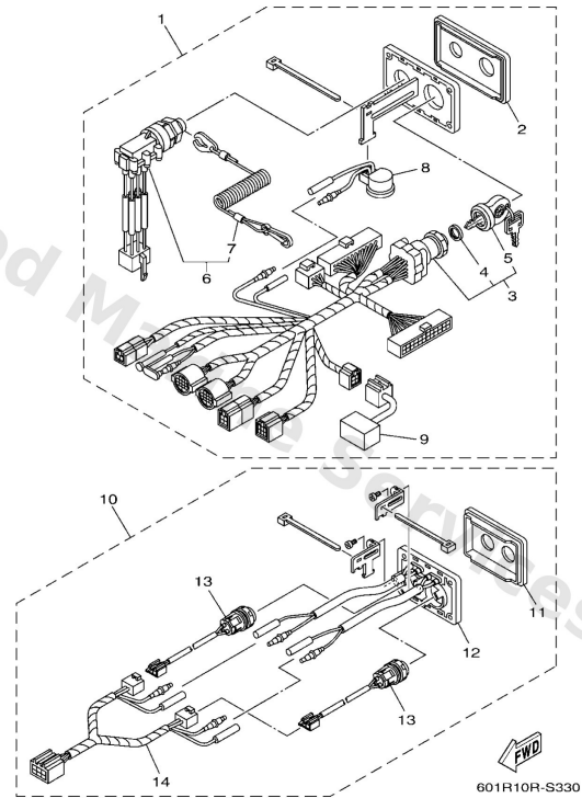
DIGITAL NETWORK SYSTEM-6Y9 (TWIN : 1 & 2 STATION-MAIN)
