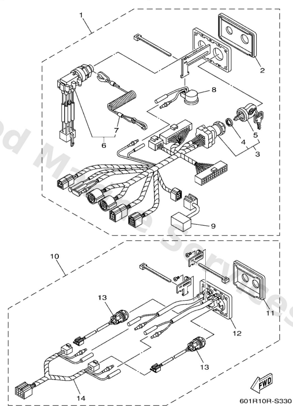
DIGITAL NETWORK SYSTEM-6Y9 (TWIN : 1 & 2 STATION-MAIN)
