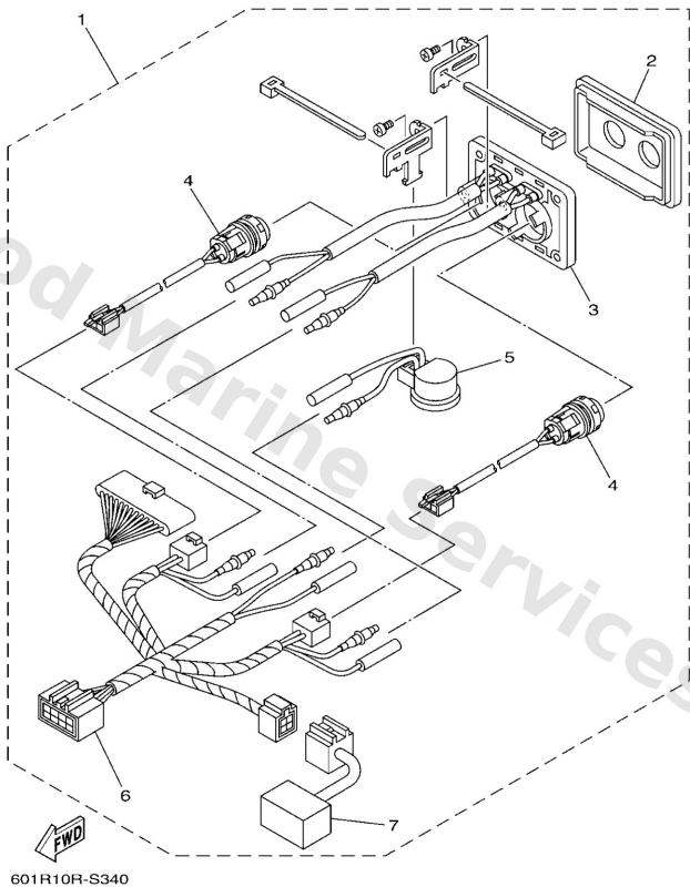
DIGITAL NETWORK SYSTEM-6Y9 (TWIN : 2 STATION-SUB)
