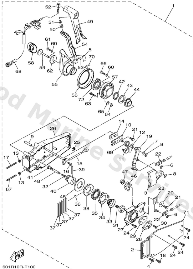
6X3 REMOTE CONTROL (LEFT MOUNT)
