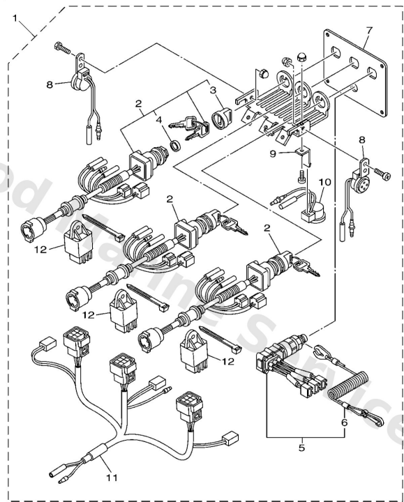
TRIPLE IG SWITCH (FOR DIGITAL NETWORK SYSTEM-6Y8)
