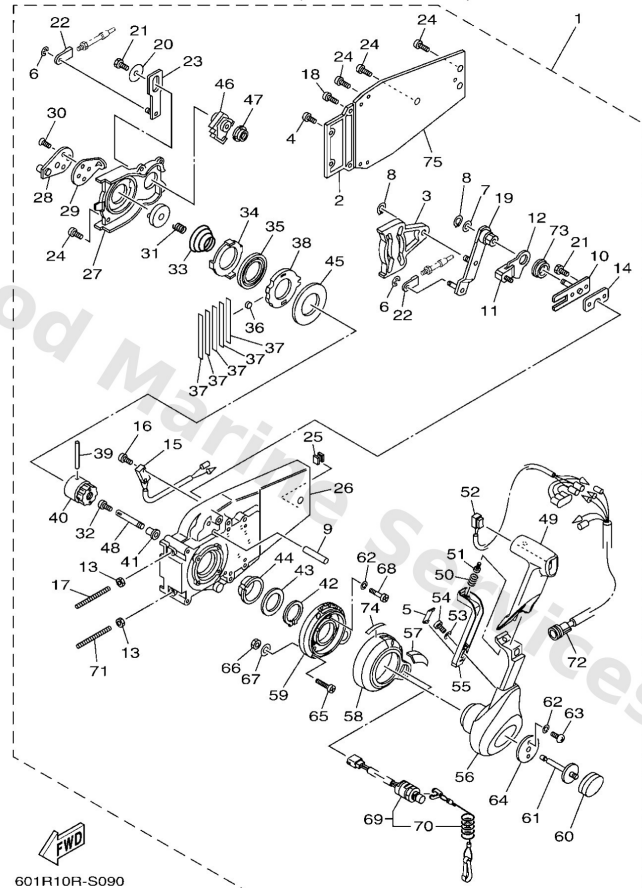
6X3 REMOTE CONTROL (RIGHT MOUNT)
