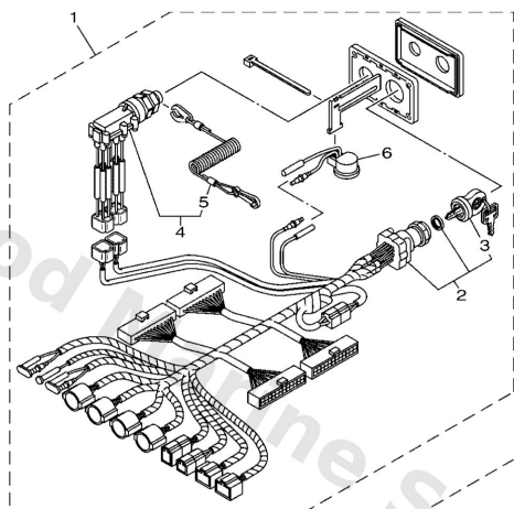
DIGITAL NETWORK SYSTEM-6Y9 (QUAD : 1 & 2 STATION-MAIN)
